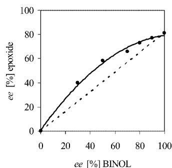
Figure 1. Asymmetric amplification in the epoxidation of chalcone at c = 0.05 catalysed by the Zn–BINOL catalyst generated in situ.
