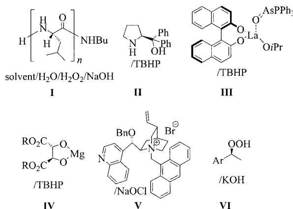
Scheme 1. Different strategies for the enantioselective epoxidation of \alpha,\beta -unsaturated ketones.
