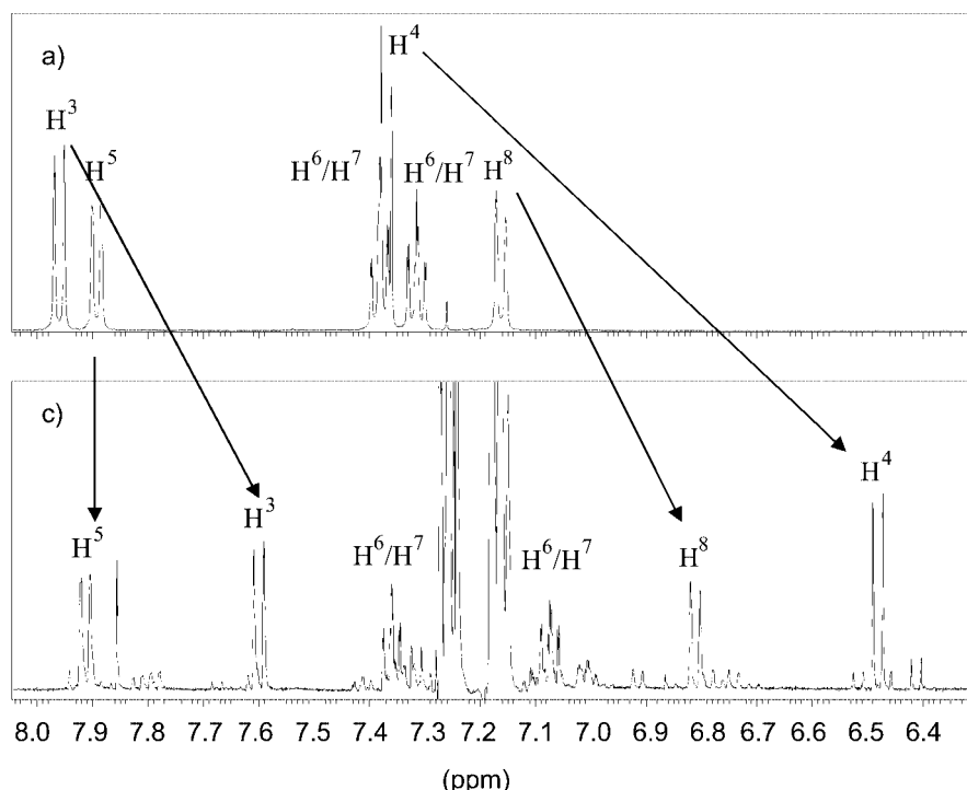
Figure 6. Enlarged aromatic sections of the ^1\text{H} NMR spectra labeled a) and c) in Figure 5.
