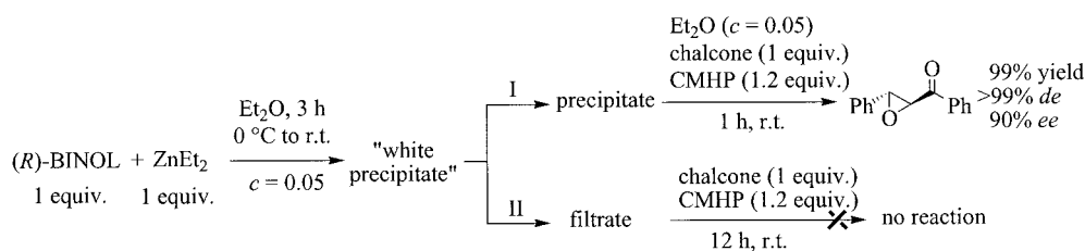
Scheme 7. Reactivity of the “white precipitate”.
