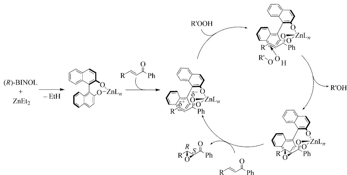
Figure 2. Proposed catalytic cycle for the enantioselective epoxidation with the Zn-( R )-BINOL catalyst.
