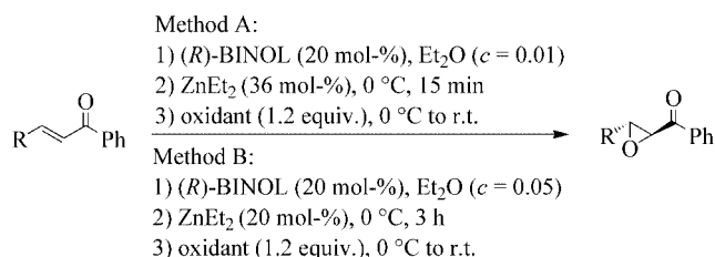
Scheme 6. Enantioselective catalytic epoxidation of alkyl-substituted enones.
