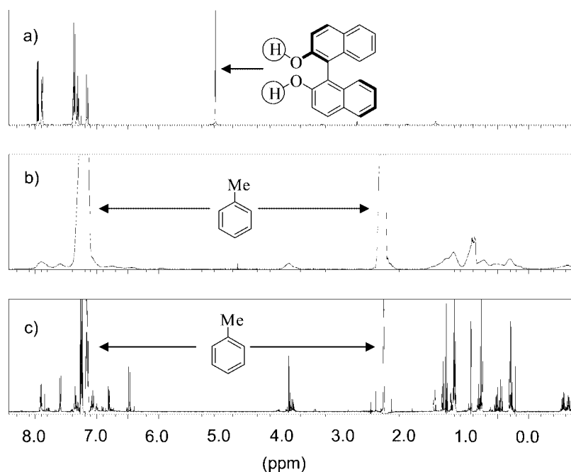
Figure 5. ^1\text{H} NMR spectrum of ( R )-BINOL ( \text{CDCl}_3 ) (a), ^1\text{H} NMR spectrum of ( R )-BINOL + 1 equiv. \text{ZnEt}_2 ( \text{CDCl}_3 , toluene) white precipitate (b), and ^1\text{H} NMR spectrum of ( R )-BINOL + 1 equiv. \text{ZnEt}_2 ( \text{CDCl}_3 , toluene) clear solution (c).
