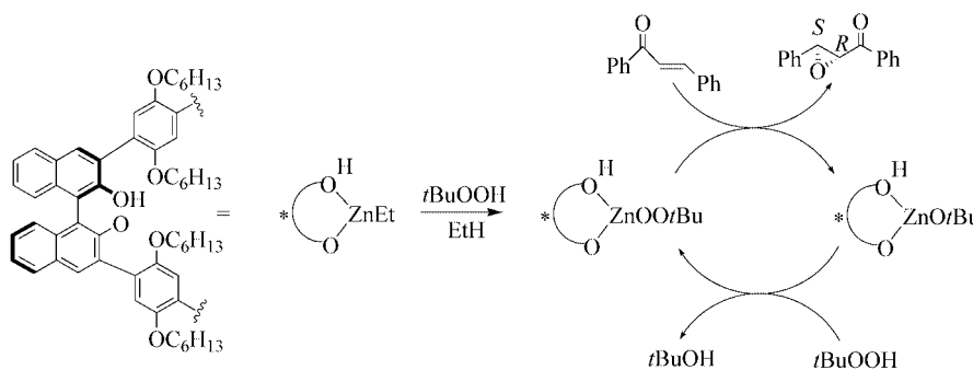
Scheme 3. Enantioselective epoxidation of enones catalysed by a chiral polybinaphthyl-zinc complex.
