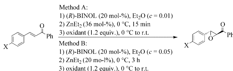
Scheme 5. Enantioselective catalytic epoxidation of substituted chalcones.
