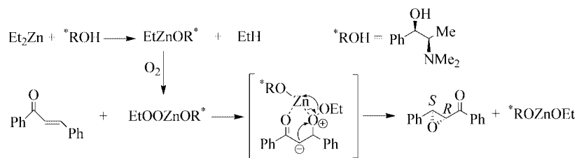
Scheme 2. Zinc-mediated aerobic enantioselective epoxidation in the presence of ( R,R )- N -methylpseudoephedrine.
