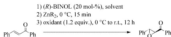
Scheme 4. Enantioselective catalytic epoxidation of chalcone.
