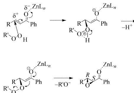
Figure 4. Proposed mechanism for the oxygen transfer.
